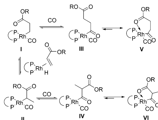
Scheme 1. Coordination of a carbonyl group to the rhodium.
