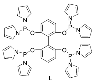
Figure 1. Ligand used in this study.
